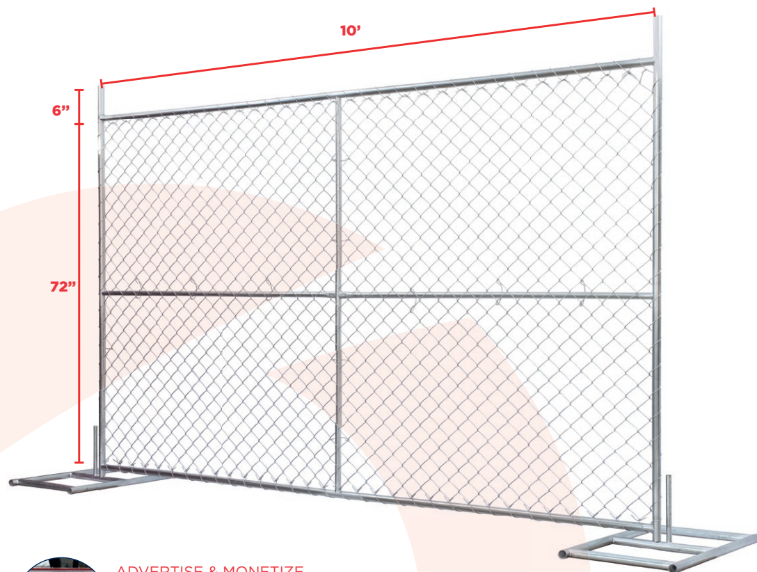
Steel Stand
